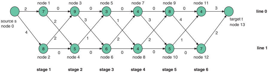
Fig. 2.1. Instance of an Assembly Line Balancing Problem
