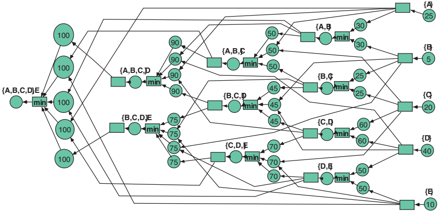
Fig. 6.1. Low-level Bellman net in its initial marking for BST
