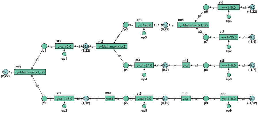
Fig. 6.18. High-level Bellman net in its final marking for KS01
