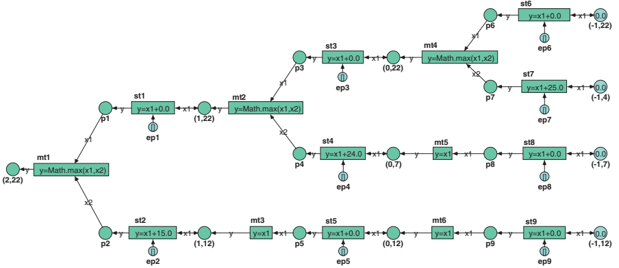
Fig. 6.17. High-level Bellman net in its initial marking for KS01
